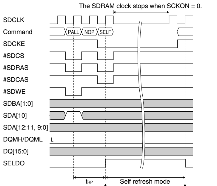
Figure II.4.1.5.7 Self Refresh
