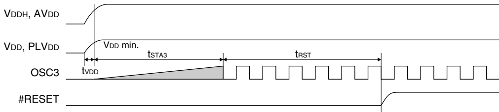
Figure I.4.6.1 Power-On Sequence
