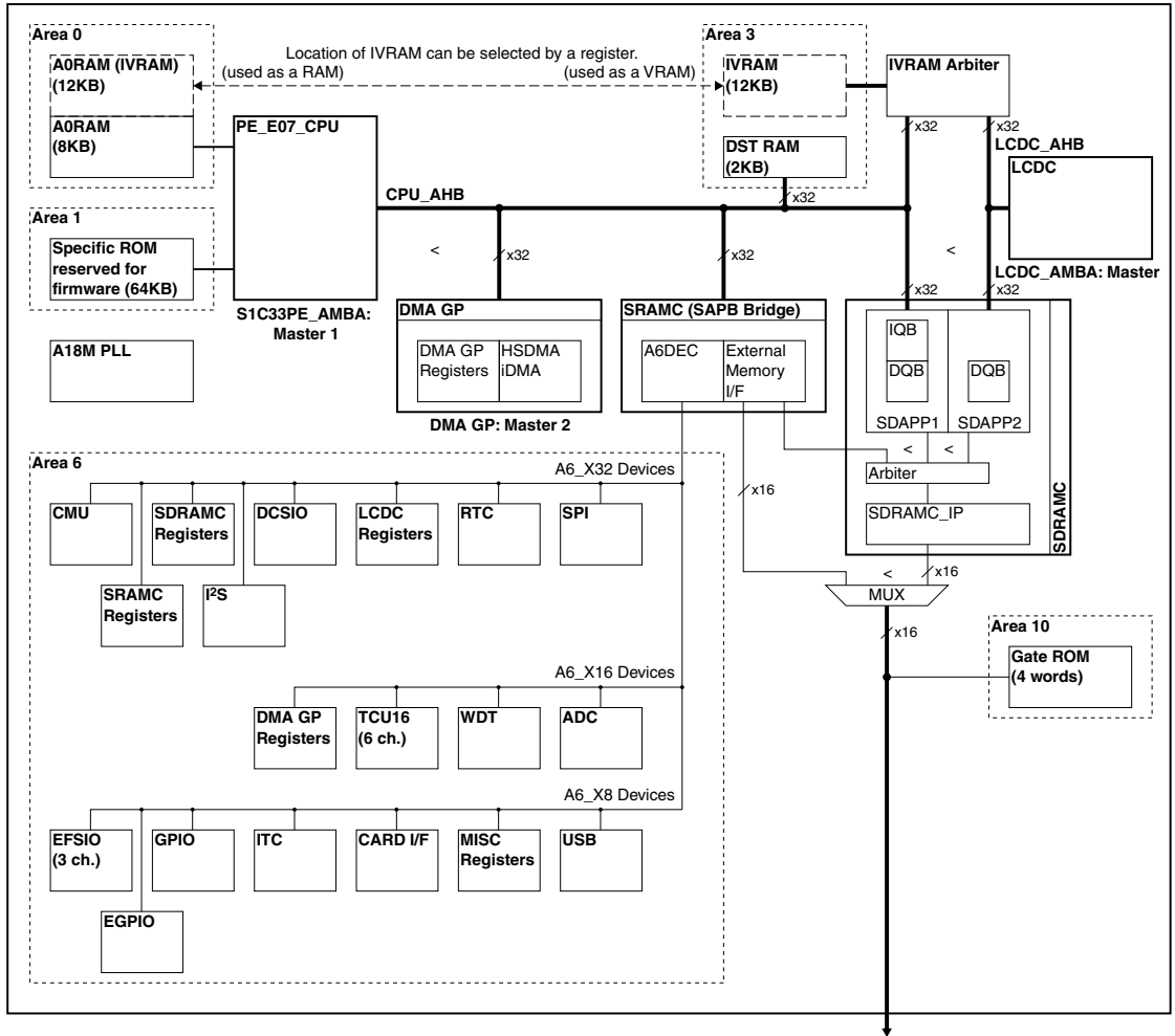
Figure I.2.1 S1C33E07 Block Diagram
