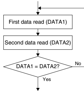
Figure III.3.3.6.1 Procedure for Reading Counters not in the Hold State
