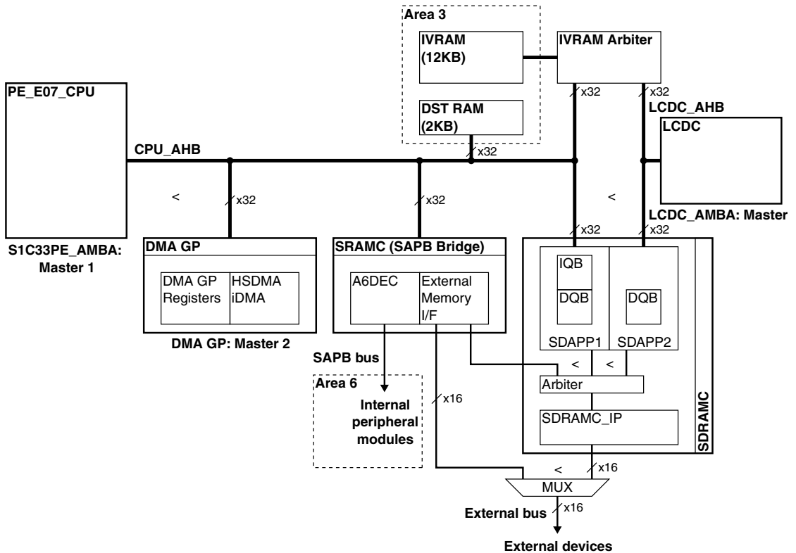
Figure I.5.7.1 S1C33E07 Bus Architecture
