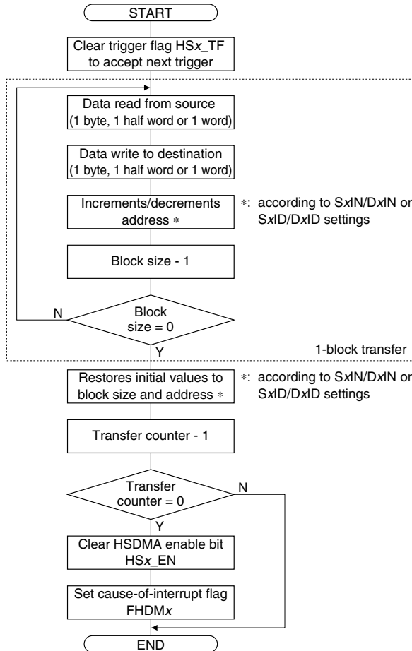
Figure II.1.6.1.3 Operation Flow in Block Transfer Mode
