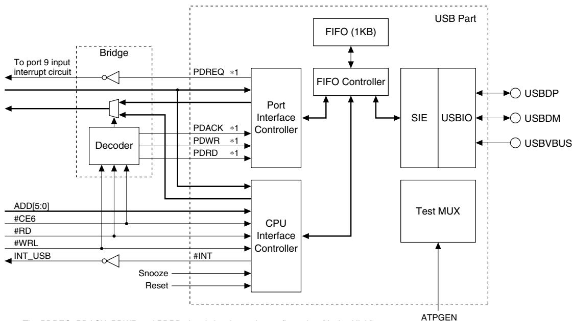
Figure IX.1.1.1 USB Function Controller Block Diagram
