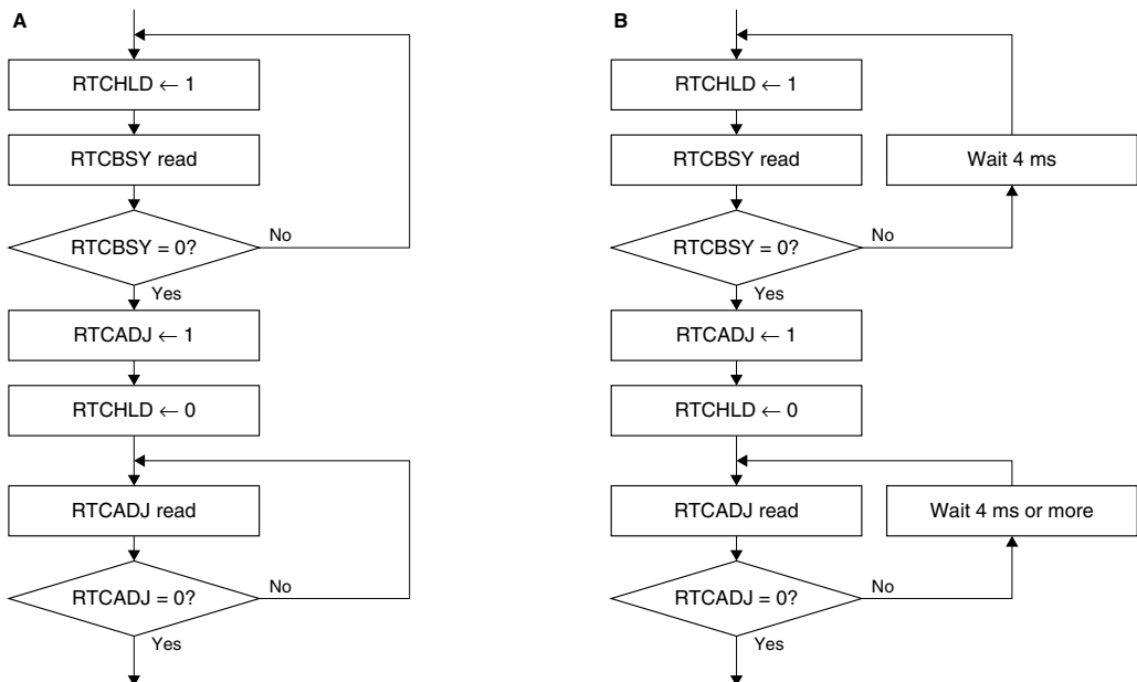
Figure III.3.3.7.1 Procedure for Executing 30-second Correction
