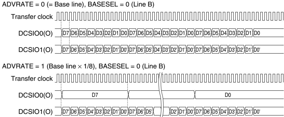
Figure V.3.4.1 DCSIO Data Formats (MSB First)
