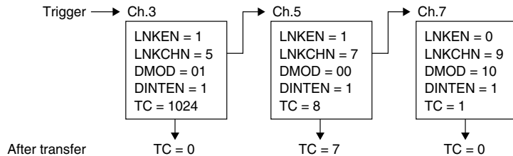
Figure II.2.5.1 Example of Link Setting
