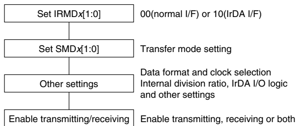
Figure V.1.9.1 Serial Interface Initialize Procedure
