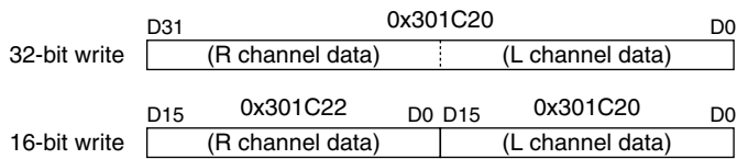
Figure V.5.7.5 Writing to FIFO
