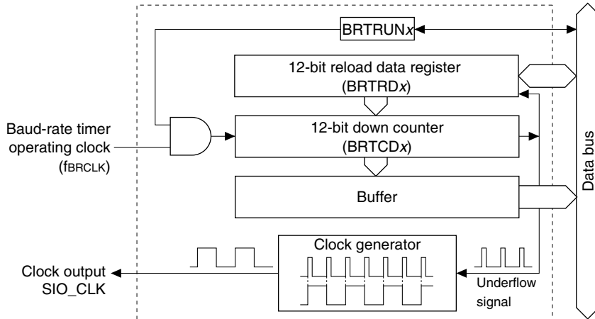
Figure V.1.2.1 Transfer Clock Generation by the Baud-Rate Timer
