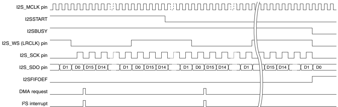
Figure V.5.5.2 Data Output Timing Chart
