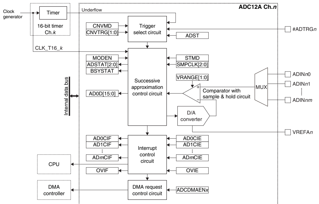
Figure 20.1.1 ADC12A Configuration
