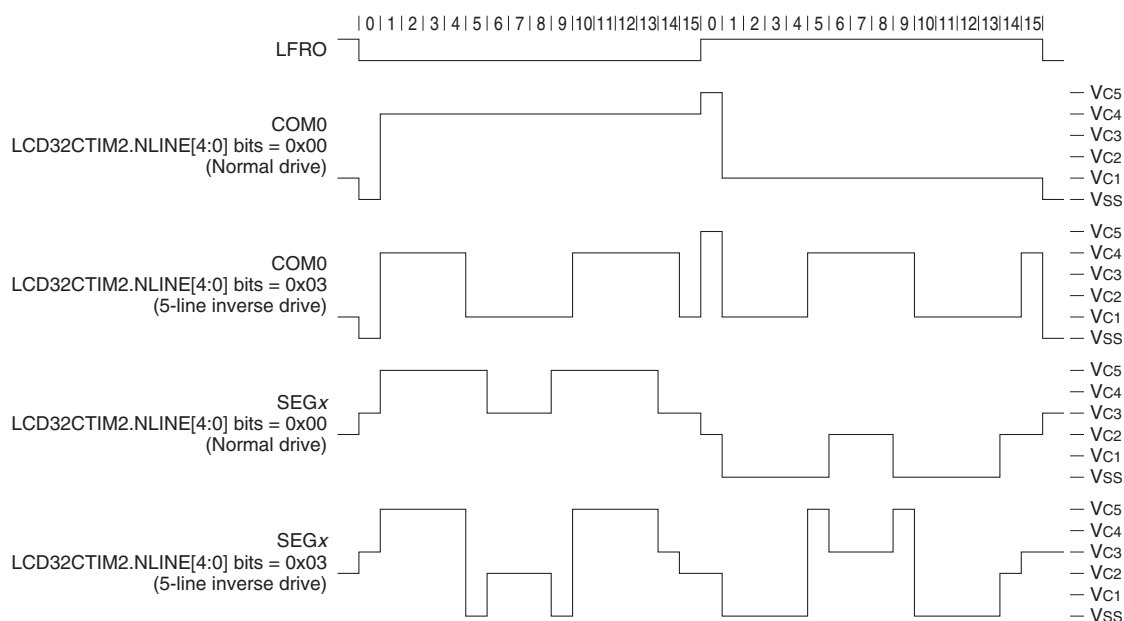
Figure 22.5.7.1 1/16 Duty Normal Drive Waveform and 5-line Inverse Drive Waveform (1/5 bias)
