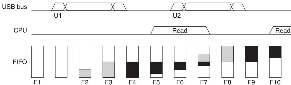
Figure 24.5.6.1 Example of Data Flow in OUT Transfer
