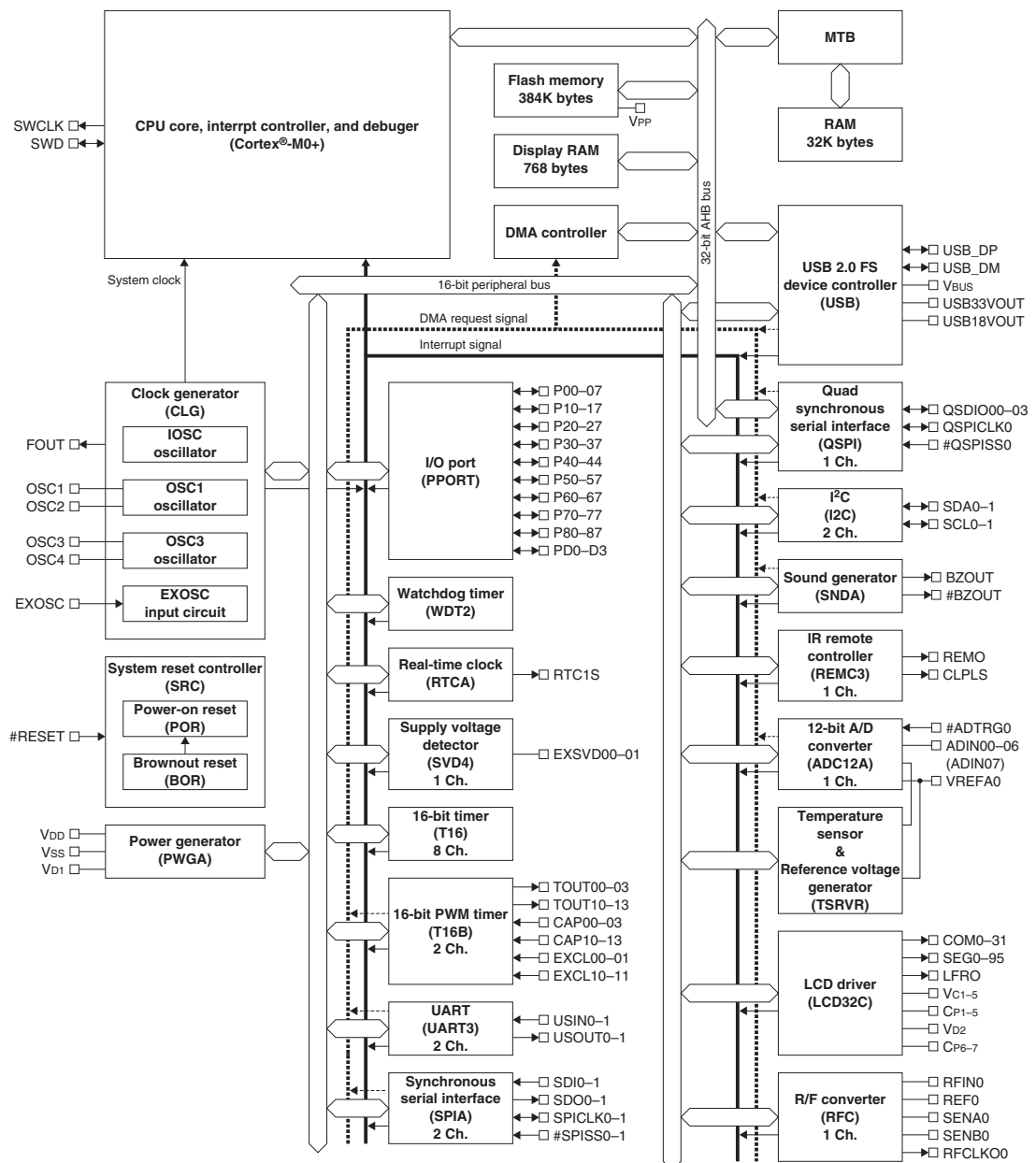
Figure 1.2.1 S1C31W73 Block Diagram
