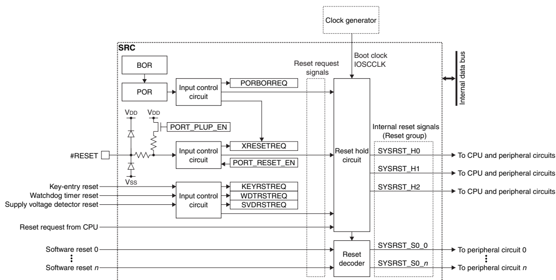
Figure 2.2.1.1 SRC Configuration
