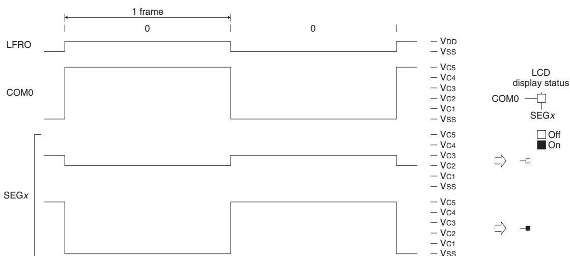
Figure 22.5.5.7 Static Drive Waveform (1/5 bias)
