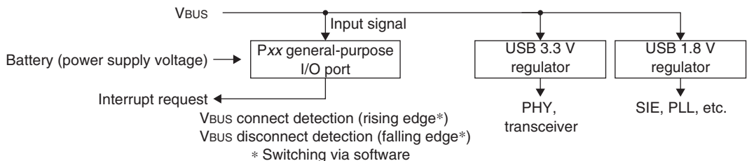
Figure 24.4.1 USB Power System
