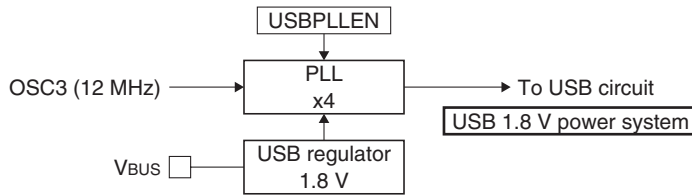
Figure 24.3.1 USB Clock System
