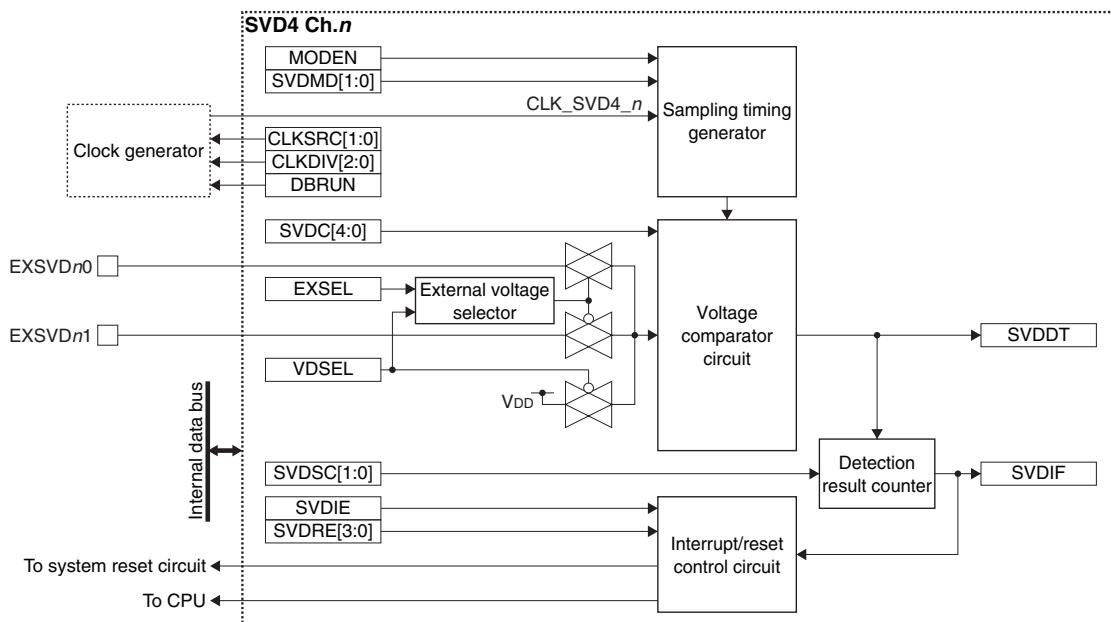
Figure 11.1.1 SVD4 Configuration
