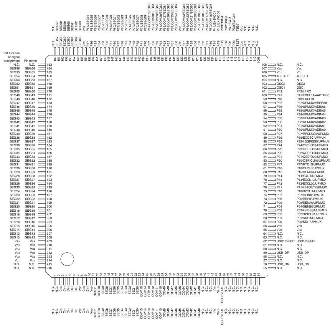
Figure 1.3.1.1 S1C31W73 Pin Configuration Diagram (QFP21-216PIN)
