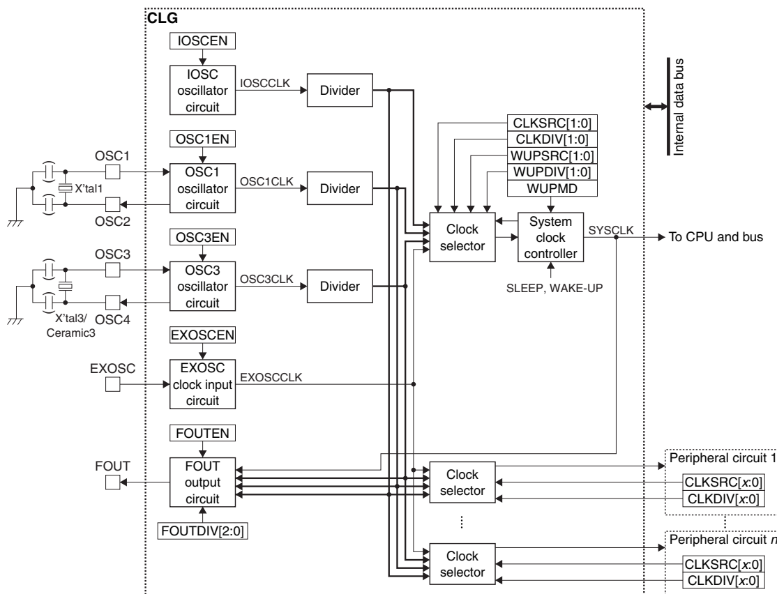
Figure 2.3.1.1 CLG Configuration
