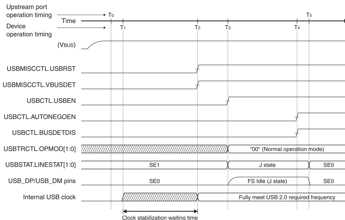
Figure 24.5.8.3 Device Attach Timing
