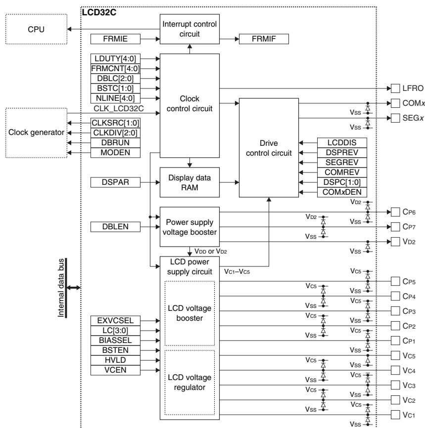
Figure 22.1.1 LCD32C Configuration
