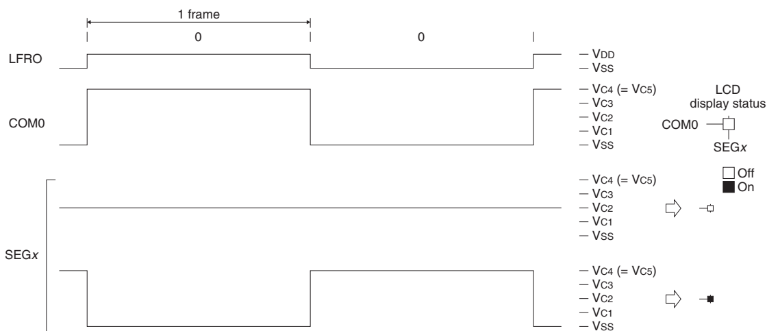
Figure 22.5.5.8 Static Drive Waveform (1/4 bias)
