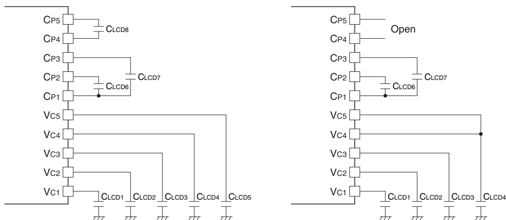
Figure 22.4.1.1 External Connection Example for Internal Generation Mode
