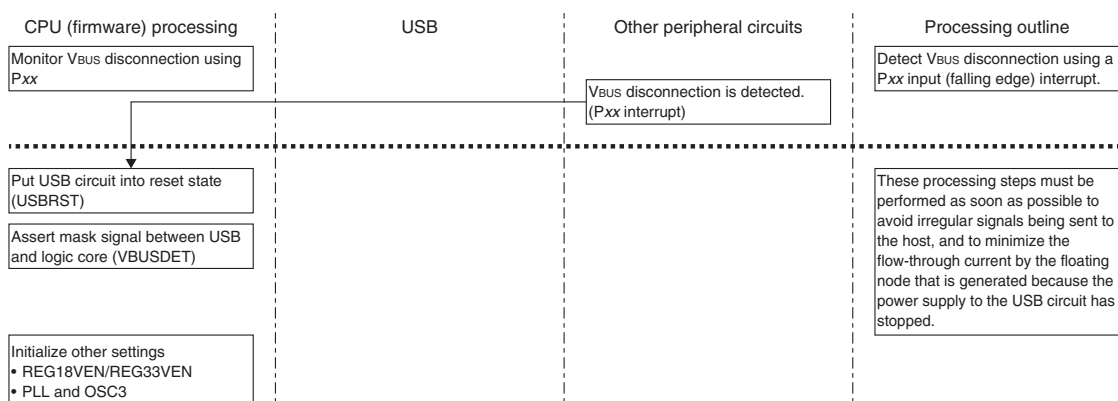
Figure 24.5.2.1 Processing Flow when VBUS is Disconnected
