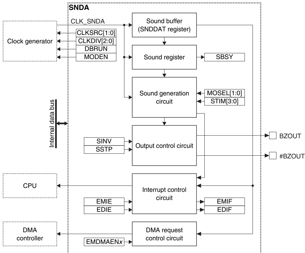
Figure 18.1.1 SNDA Configuration
