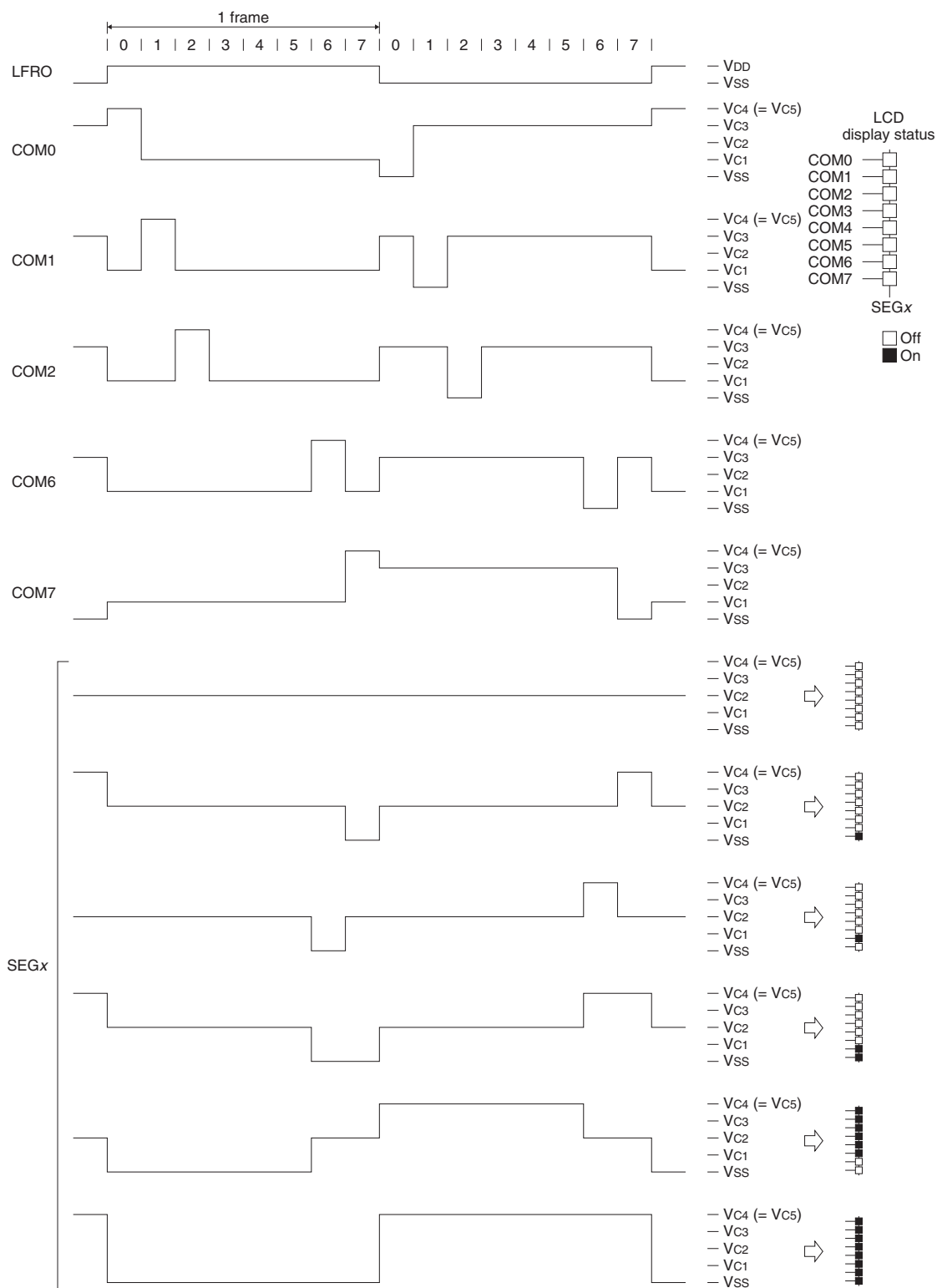
Figure 22.5.5.6 1/8 Duty Drive Waveform (1/4 bias)
