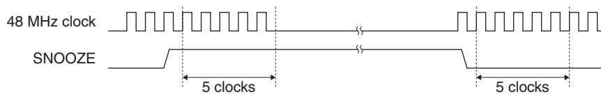
Figure 24.5.10.1 Snooze Sequence
