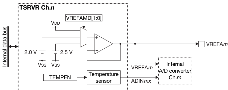
Figure 21.1.1 TSRVR Configuration
