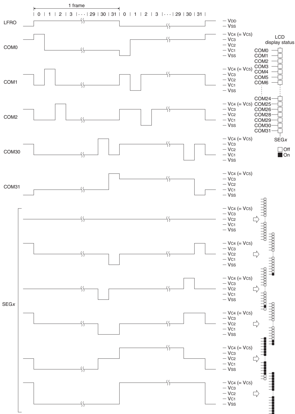
Figure 22.5.5.2 1/32 Duty Drive Waveform (1/4 bias)
