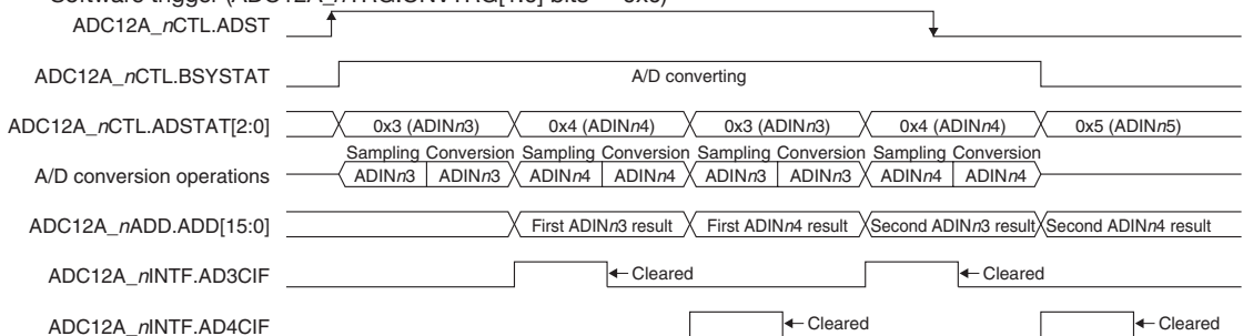
Figure 20.4.4.1 A/D Conversion Operations
