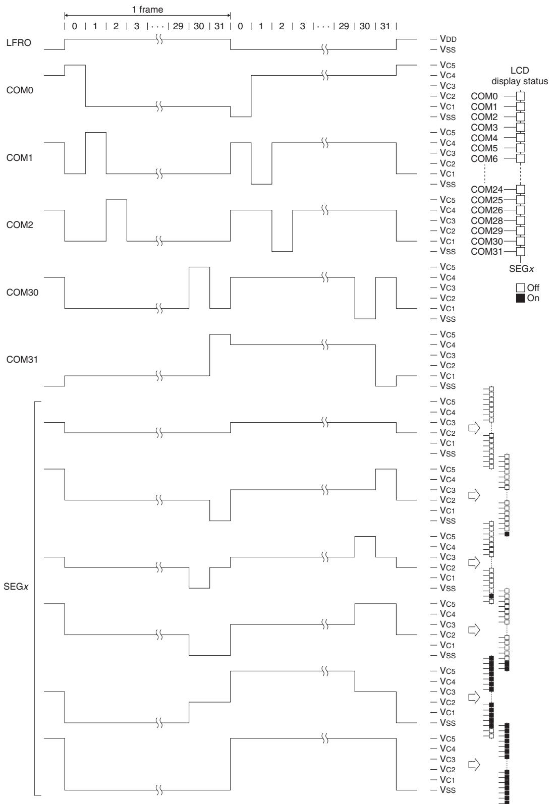
Figure 22.5.5.1 1/32 Duty Drive Waveform (1/5 bias)
