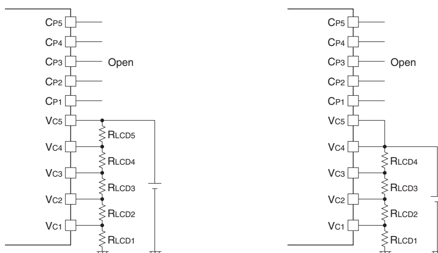
Figure 22.4.2.1 External Connection Example for External Voltage Application Mode (resistor divider)
