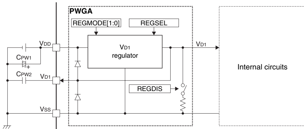
Figure 2.1.1.1 PWGA Configuration
