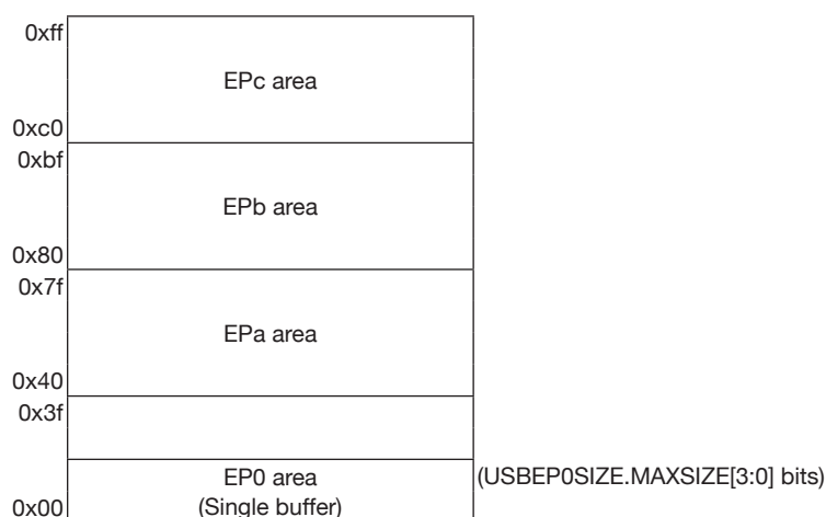
Figure 24.5.9.1 FIFO Memory Map
