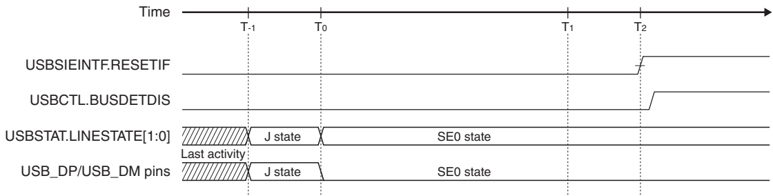
Figure 24.5.8.2 Reset Timing
