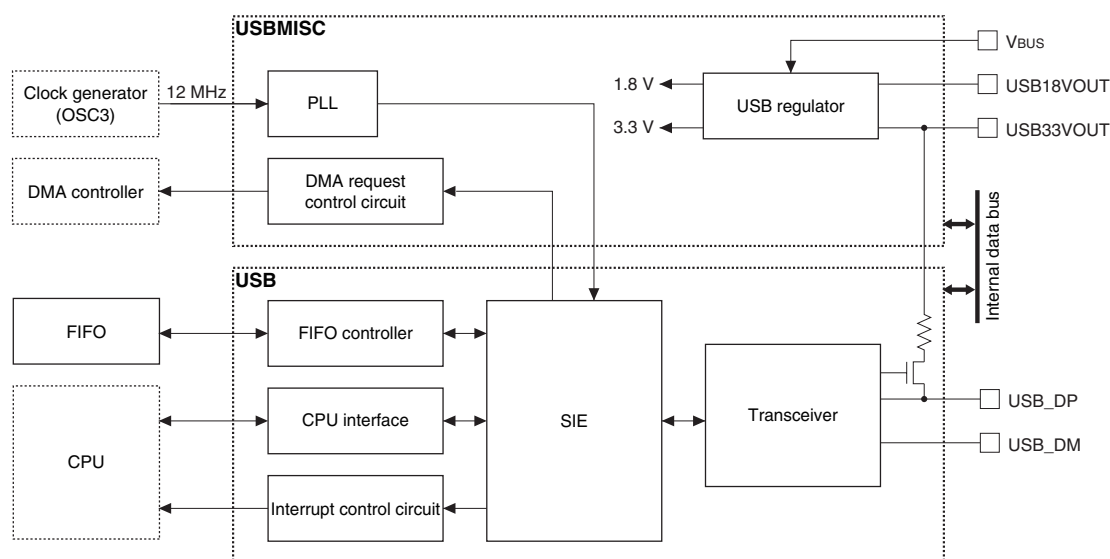
Figure 24.1.1 USB Controller Configuration
