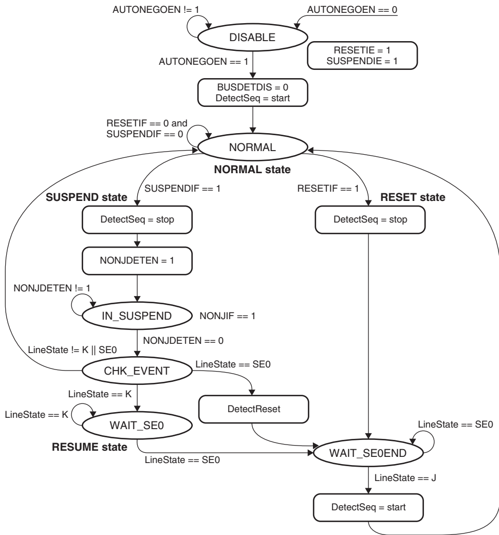
Figure 24.5.7.1 Auto-Negotiator
