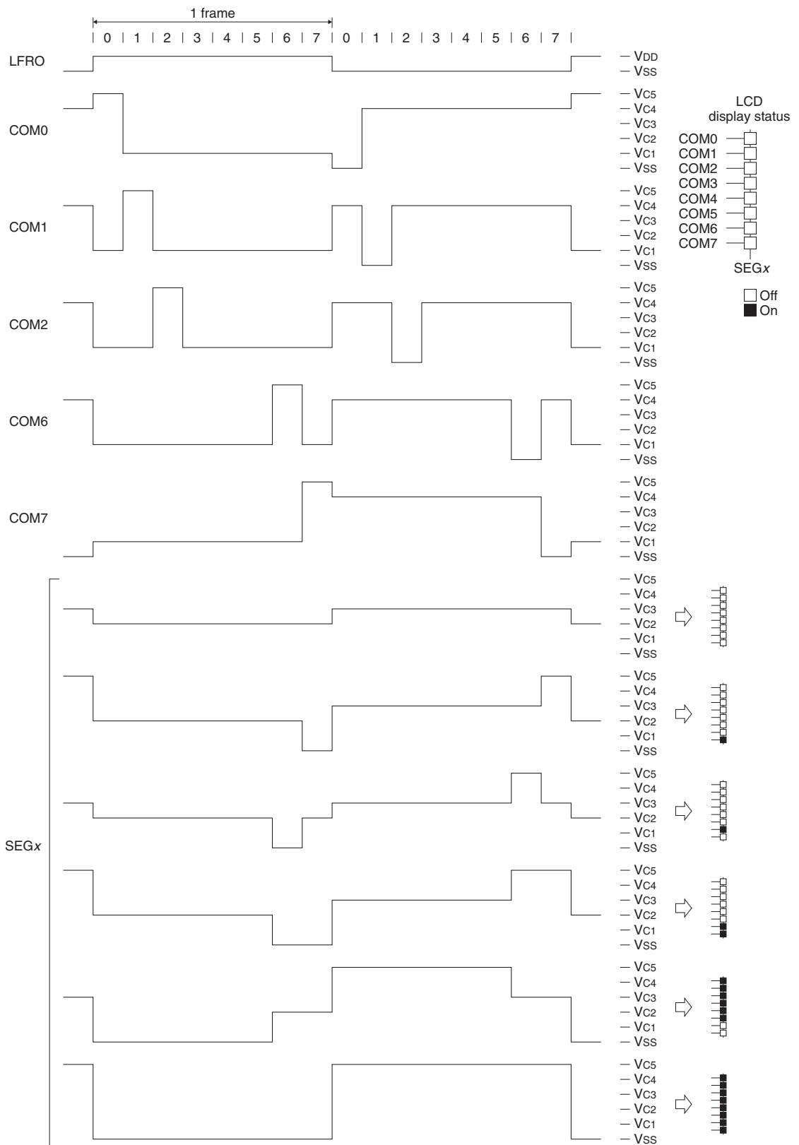
Figure 22.5.5.5 1/8 Duty Drive Waveform (1/5 bias)
