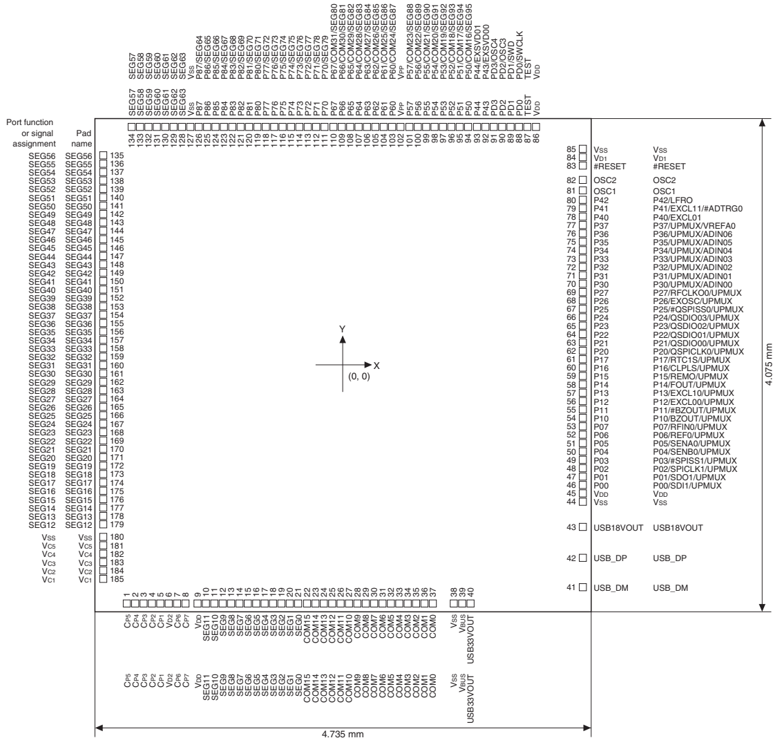
Figure 1.3.2.1 S1C31W73 Pad Configuration Diagram
