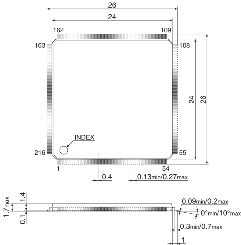
Figure 27.1 QFP21-216PIN Package Dimensions
