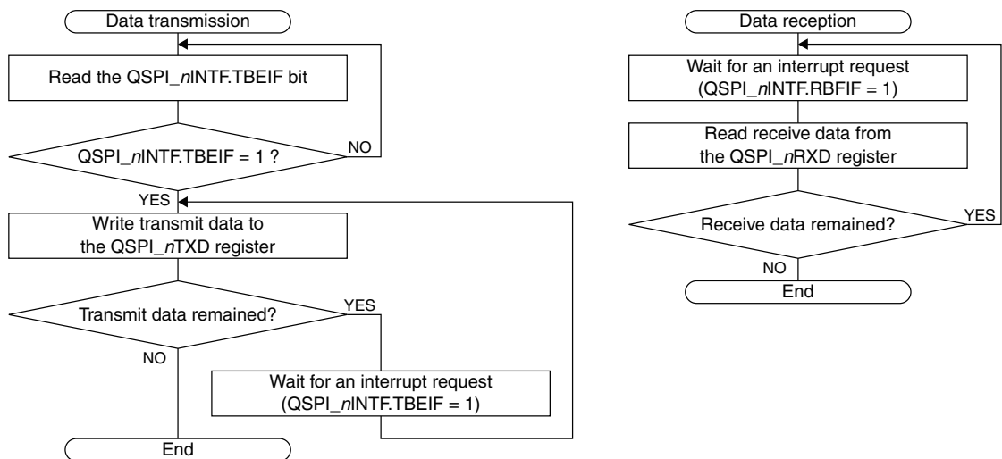
Figure 15.5.9.2 Data Transfer Flowcharts in Slave Mode
