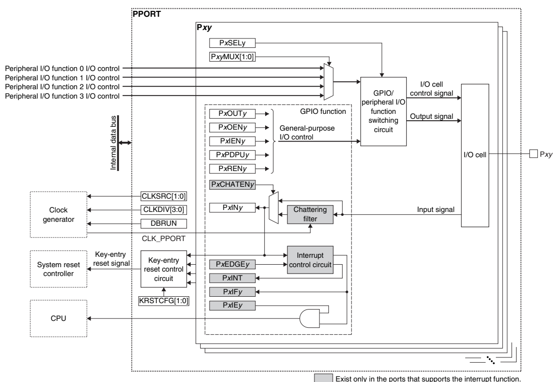
Figure 7.1.1 PPORT Configuration
