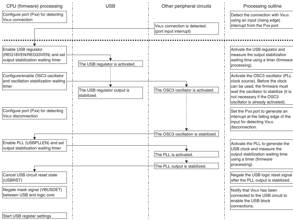
Figure 24.5.1.1 Processing flow before and after V BUS is connected
