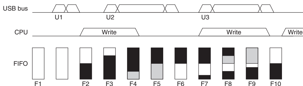
Figure 24.5.6.2 Example of Data Flow in IN Transfer
