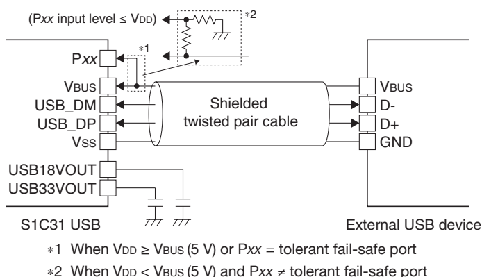
Figure 24.2.2.1 Connections between USB controller and an External USB Device
