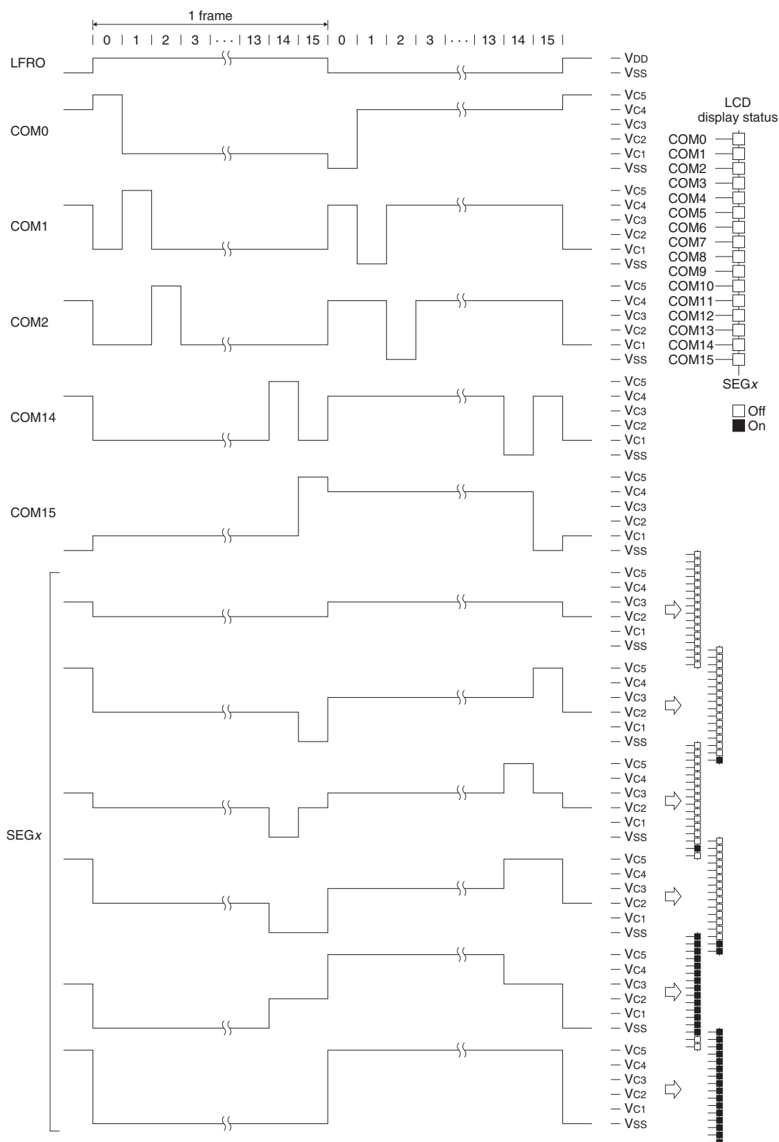
Figure 22.5.5.3 1/16 Duty Drive Waveform (1/5 bias)
