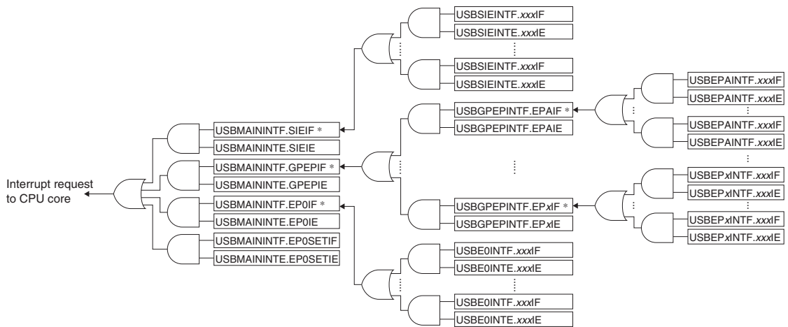
Figure 24.6.1 USB Interrupt System
