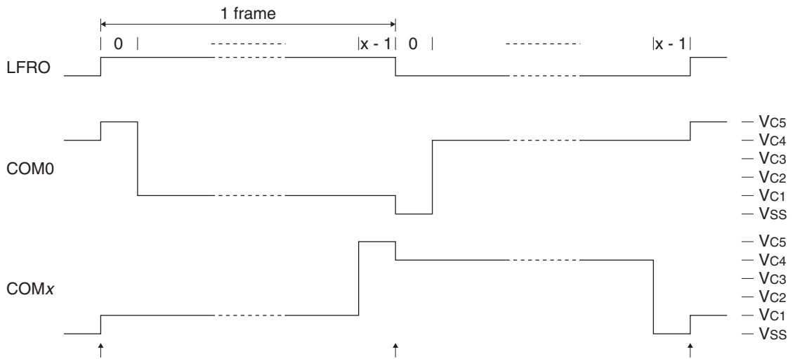
Figure 22.7.1 Frame Interrupt Timings (1/x duty, 1/5 bias)
