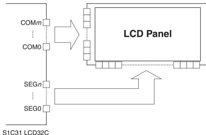
Figure 22.2.2.1 Connections between LCD32C and an LCD Panel
