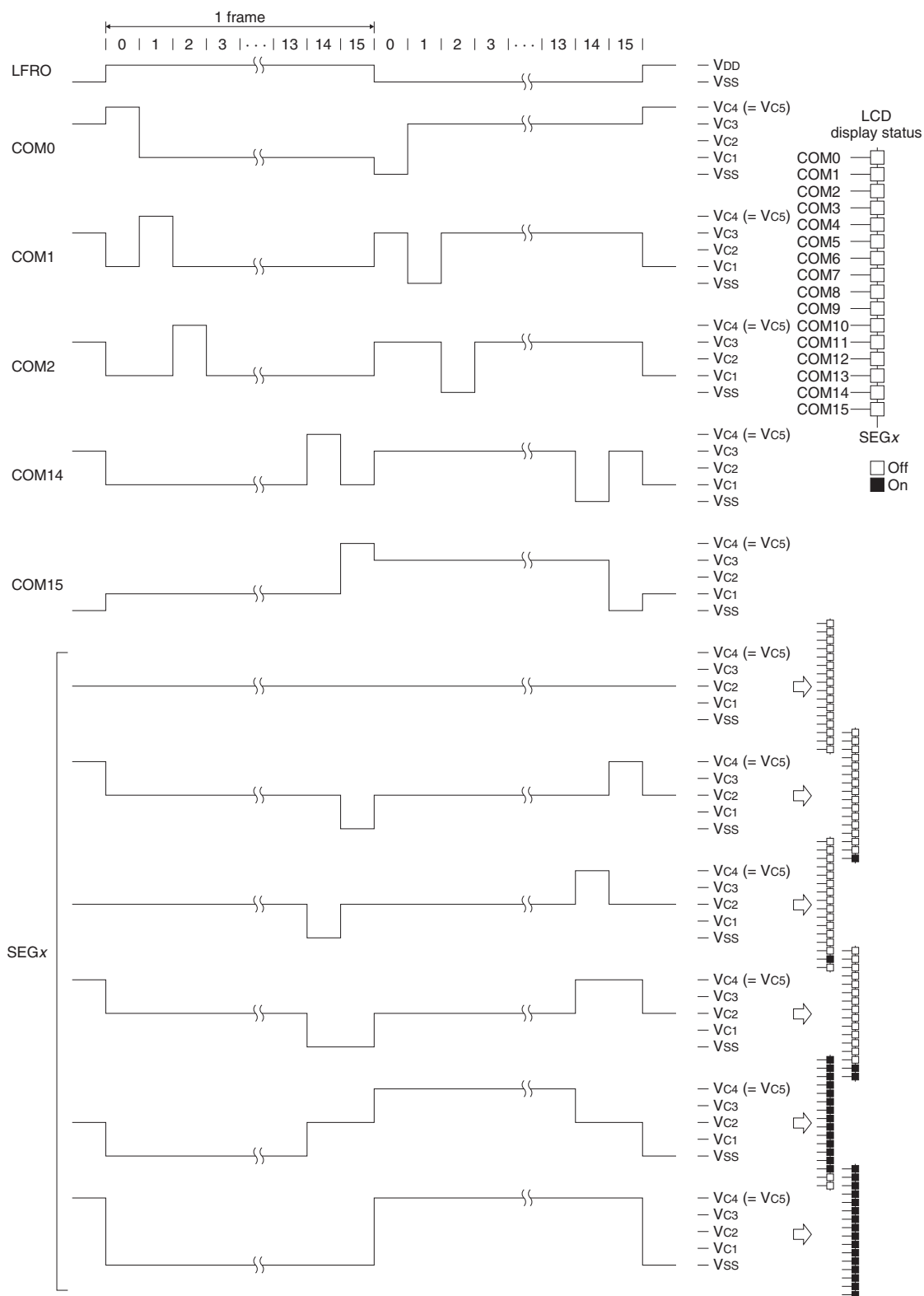
Figure 22.5.5.4 1/16 Duty Drive Waveform (1/4 bias)
