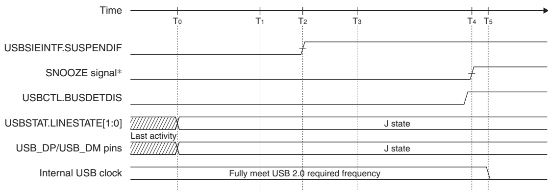
Figure 24.5.8.1 Suspend Timing
