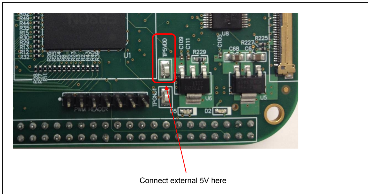
TP5VDD Location
