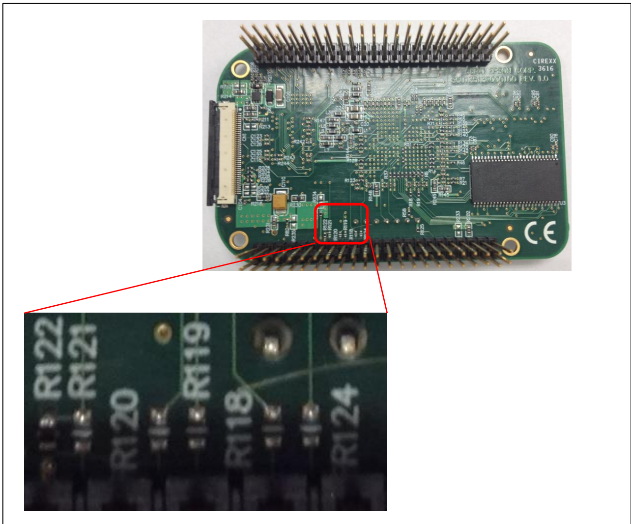
SPI Interface Modifications: Resistor Locations
