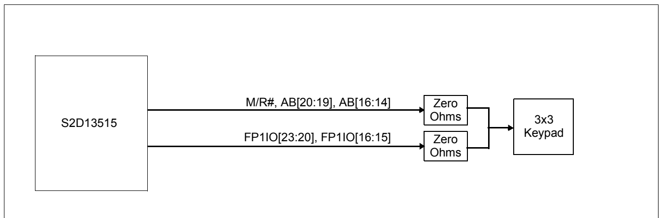
Figure 4-6: Keypad Interface Zero Ohm Resistor Overview Diagram
