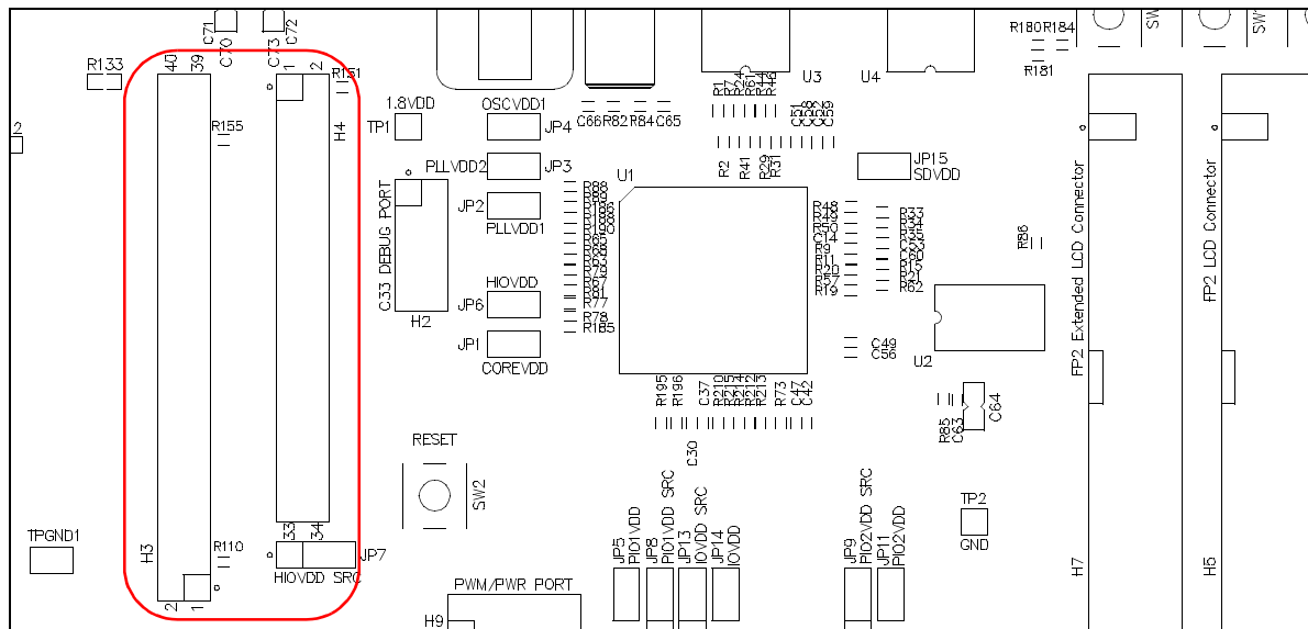
Figure 4-2: Host Bus Connector Location (H3 and H4)
