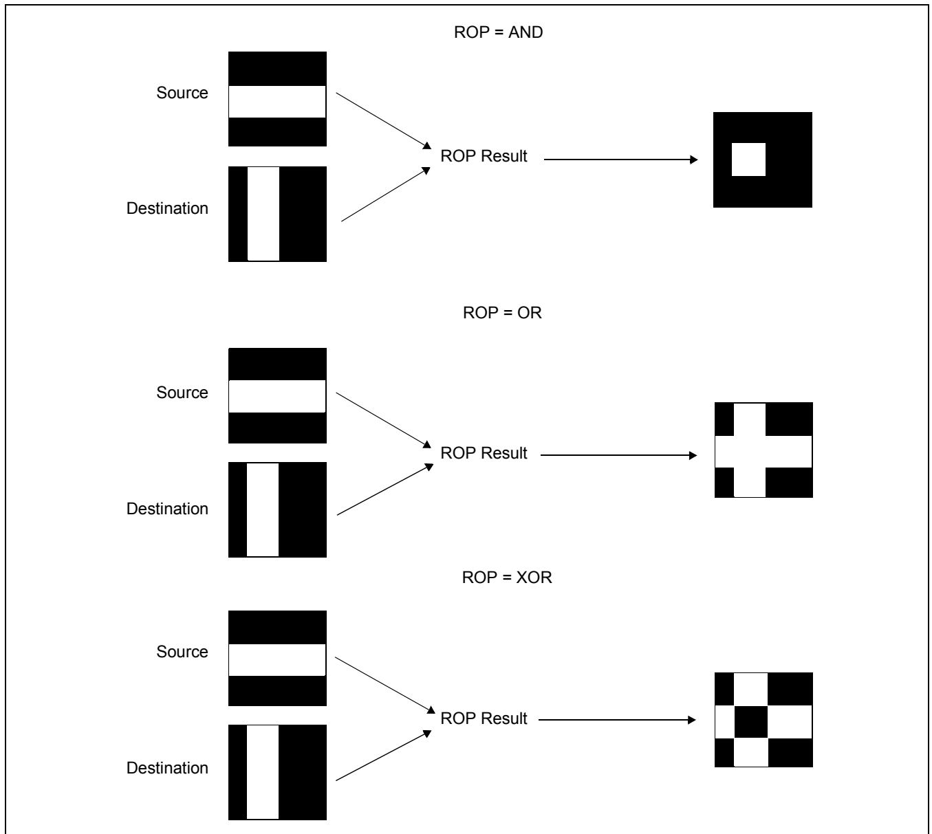
Figure 18-7: ROP Example
