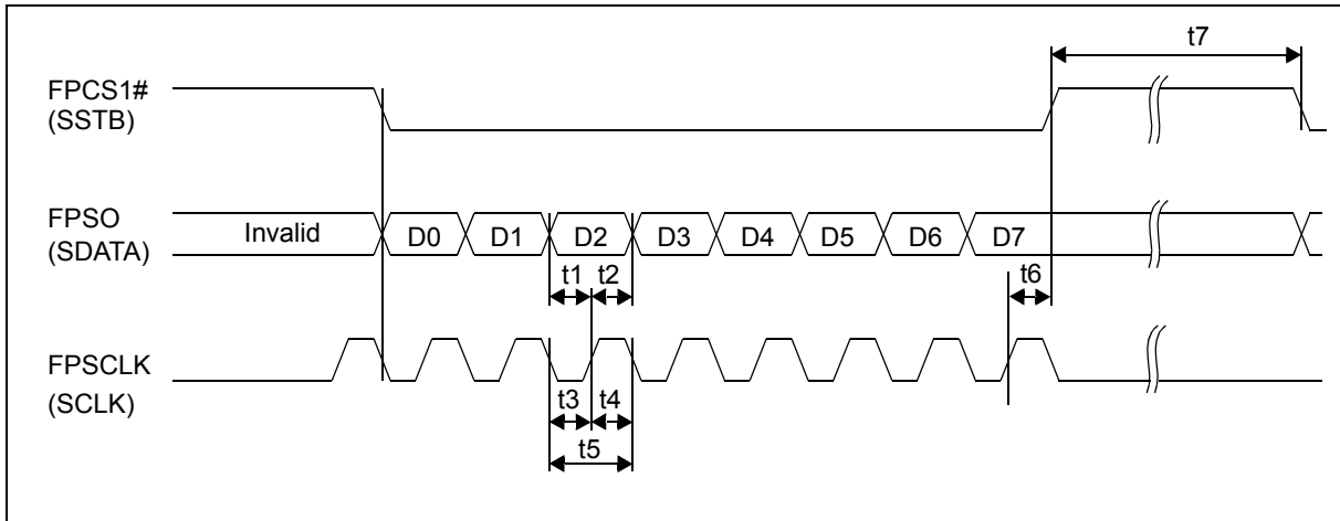
Figure 7-37: LCD1 a-Si TFT Serial Interface Timing
