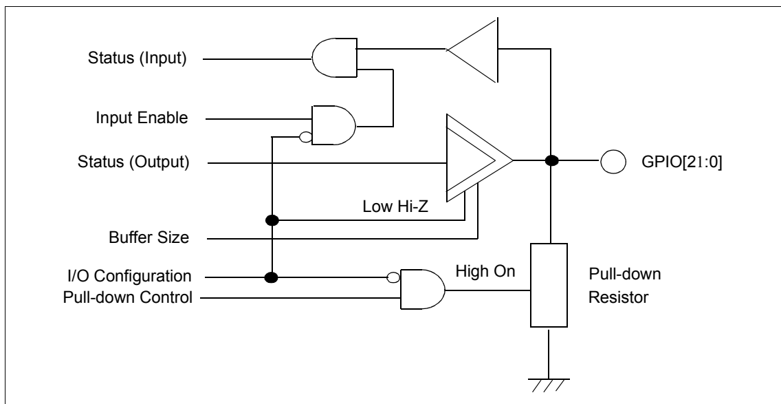
Figure 23-1: IO Cell Structure
