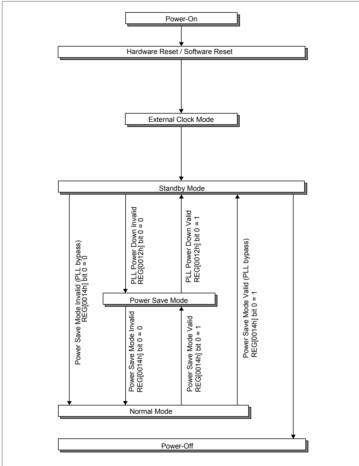
Figure 11-2: Power Modes
