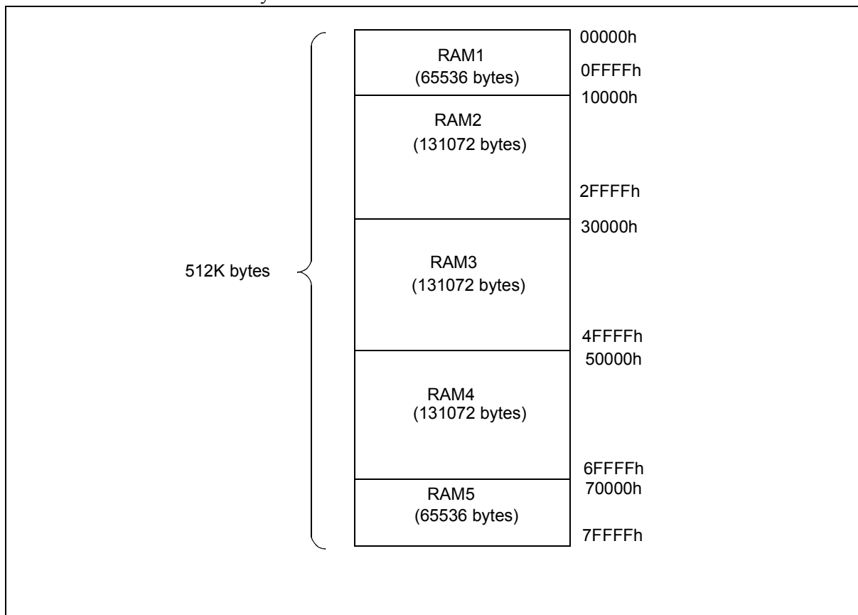
Figure 8-1: Physical Memory
