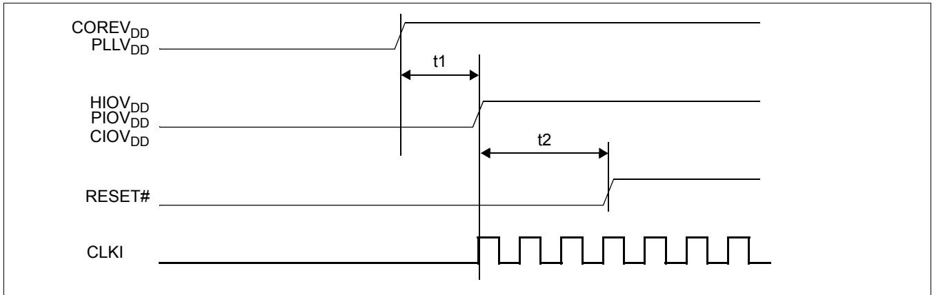
Figure 7-4: Power-On Sequence
