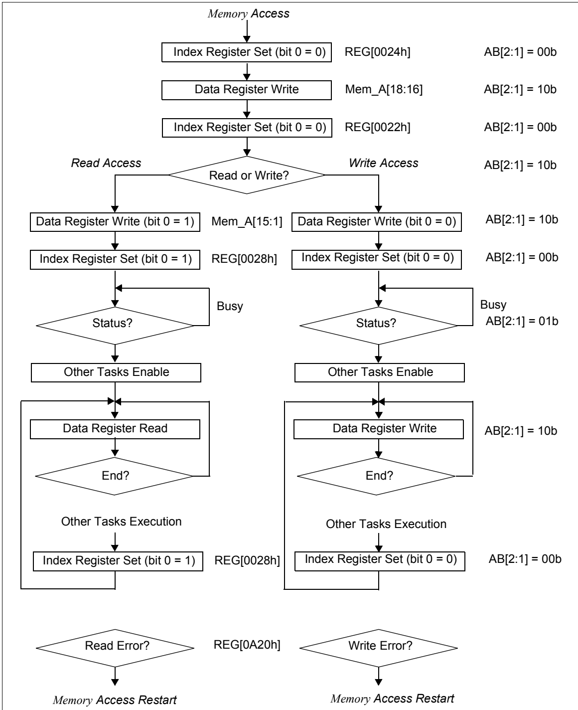
Figure 19-5: Memory Access
