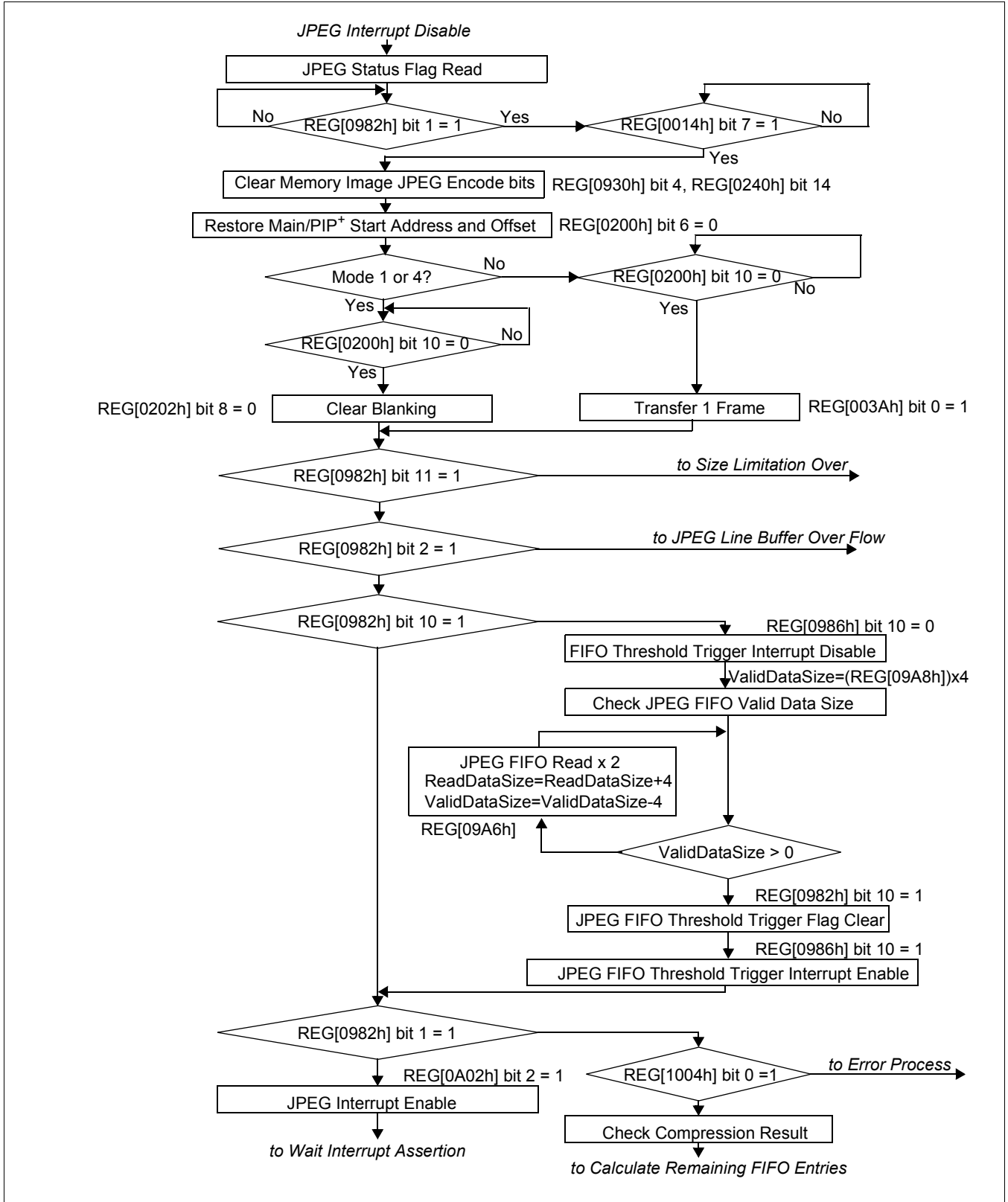
Figure 14-8: Memory Image JPEG Encoding Process (3 of 4)
