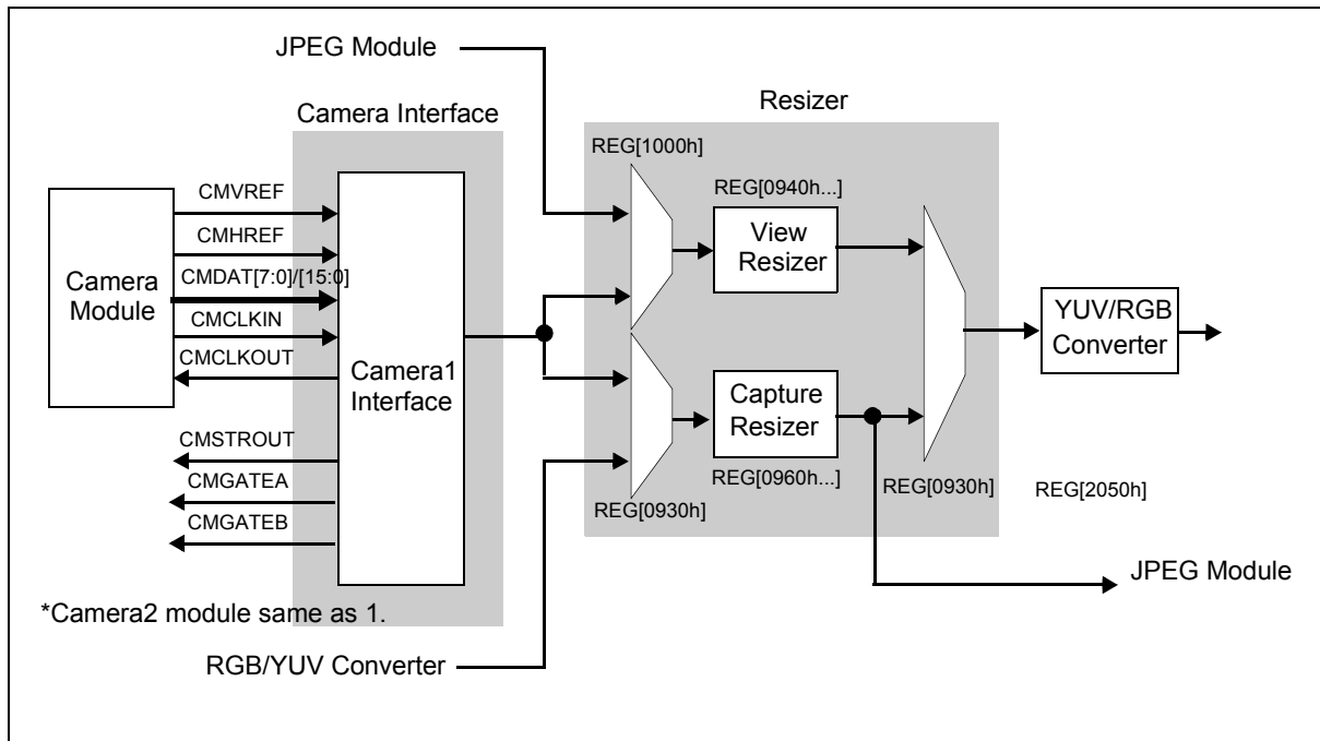
Figure 21-1: Camera Interface
