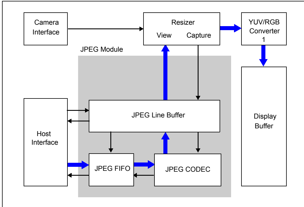
Figure 16-2: Internal JPEG Decode Data Flow
