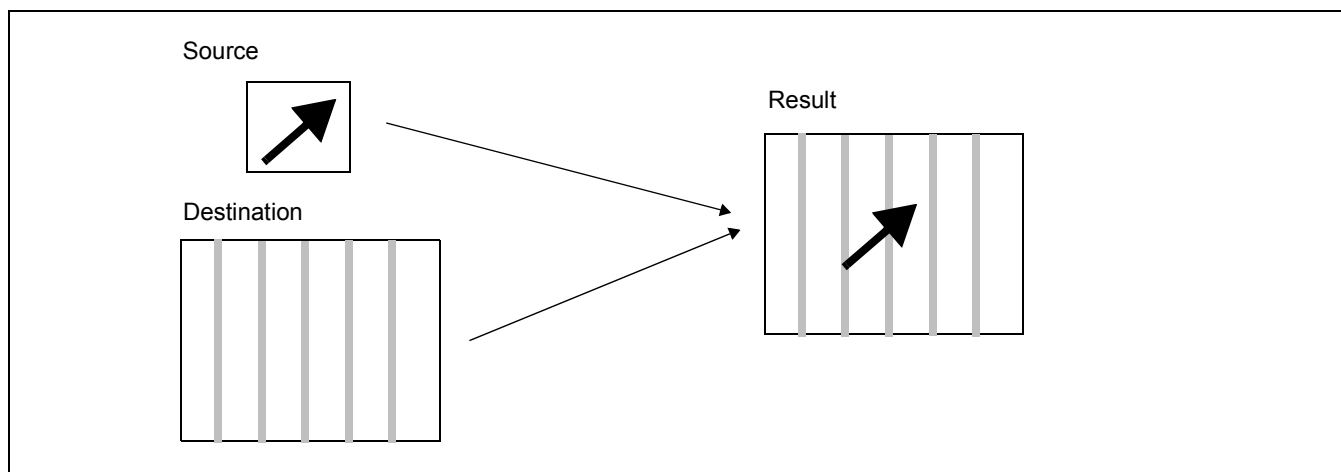
Figure 18-8: Transparency Example
