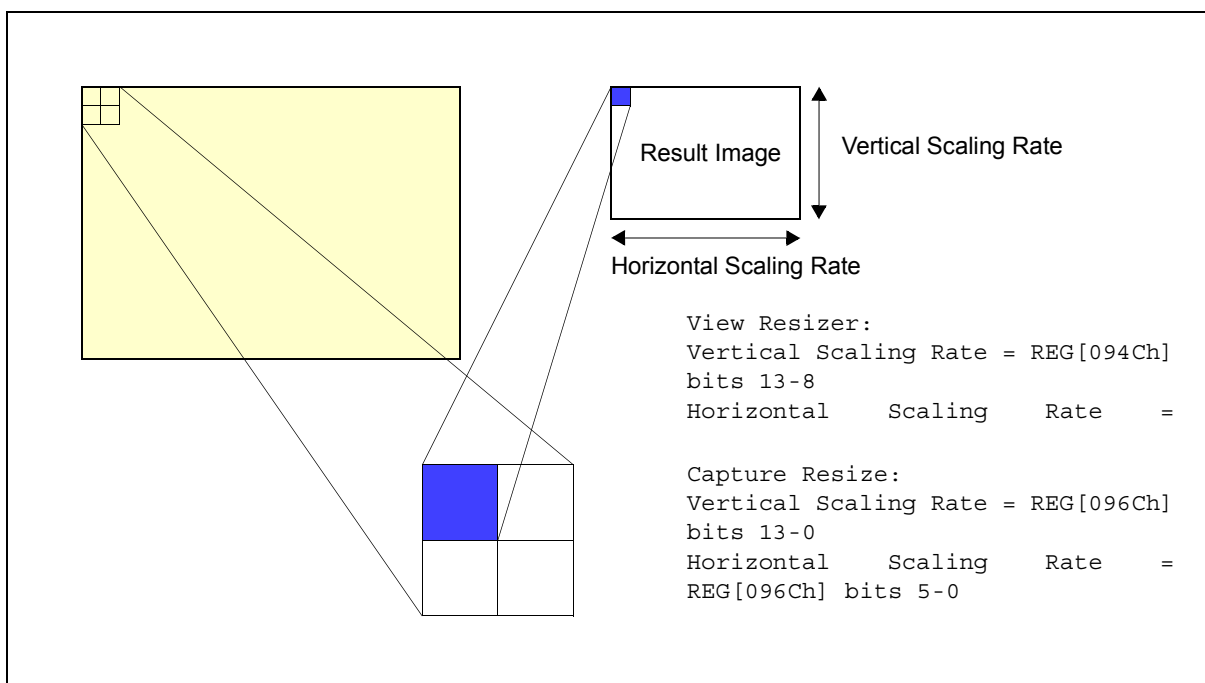
Figure 15-3: Scaling Function
