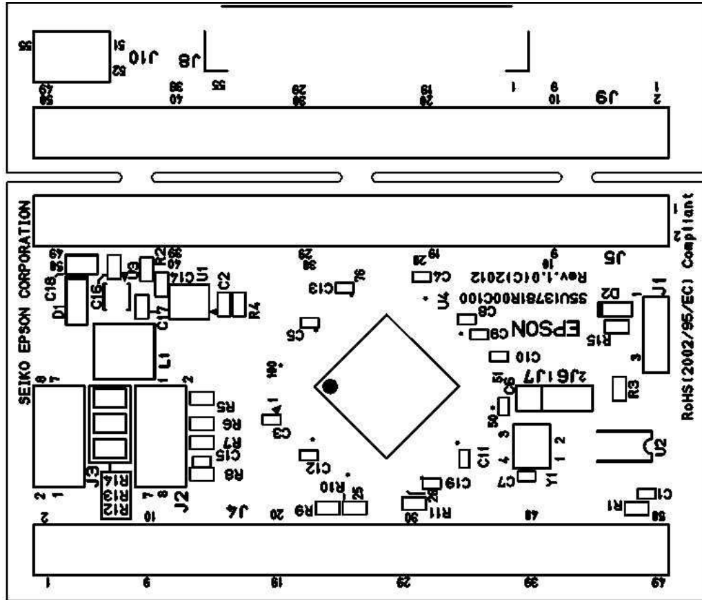
Figure 8-1 S5U13781R00C100 Board Layout Silk Screen
