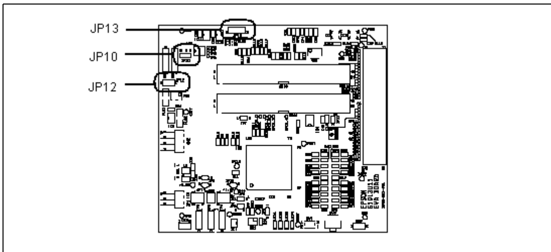
Figure 3-4: Configuration Jumper Locations (JP10, JP12, JP13)
